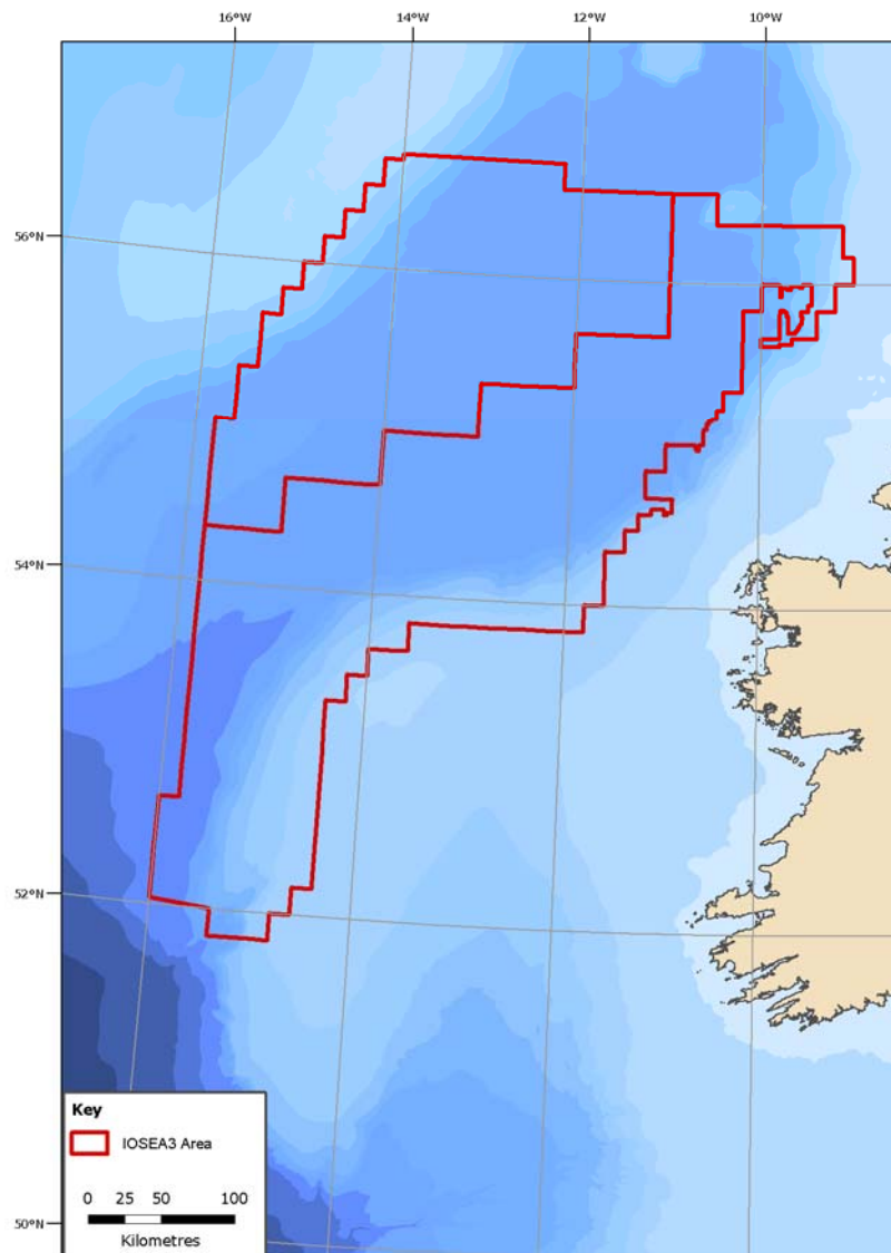
Figure 1.1 IOSEA3 area of the Rockall Basin
