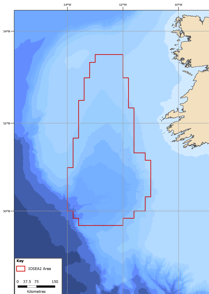
Figure 1.1 IOSEA2 area of the Porcupine Basin
